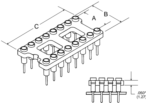
Low Profile Solder Tail Type -01
